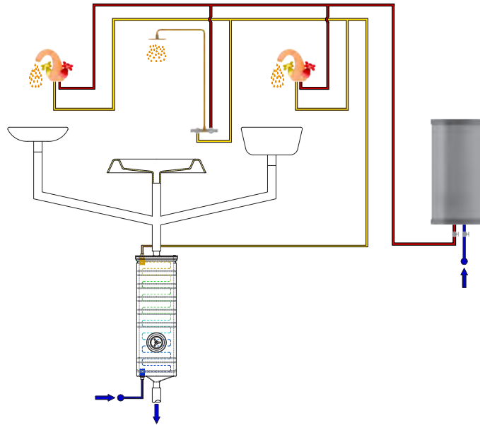
Collegamento monozona - Single-area connection Schema B recupero totale - Diagram B total recovery
