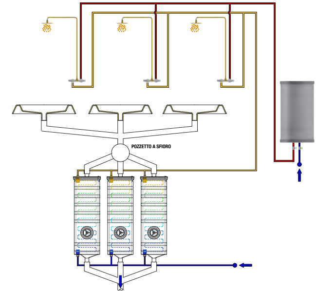
Collegamento parallelo - Parallel connection Schema A - Diagram A
