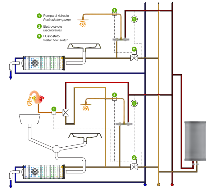
Collegamento multizona - Connecting multi-area Schema B recupero totale - Diagram B total recovery
